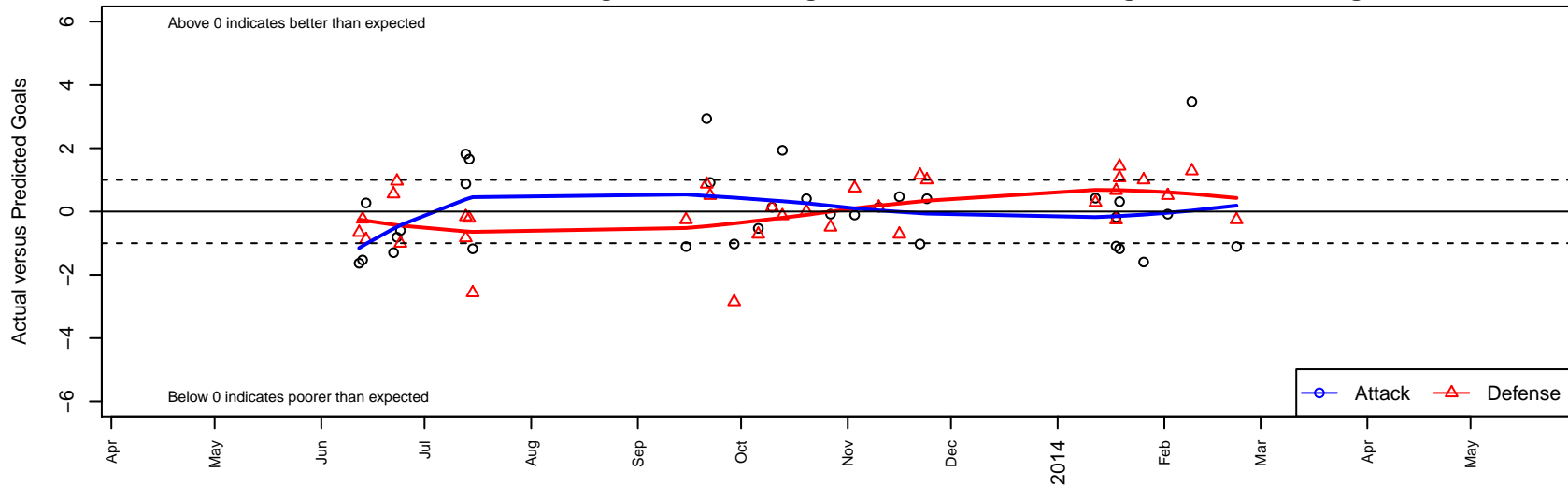
Eastside FC Red B95 Dots are actual minus expected GF (blue circles) and GA (red triangles). Blue line is smoothed change in attack strength. Red is smoothed change in defense strength.
